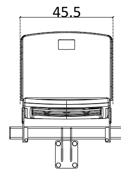
MONORAIL SINGLE-301
