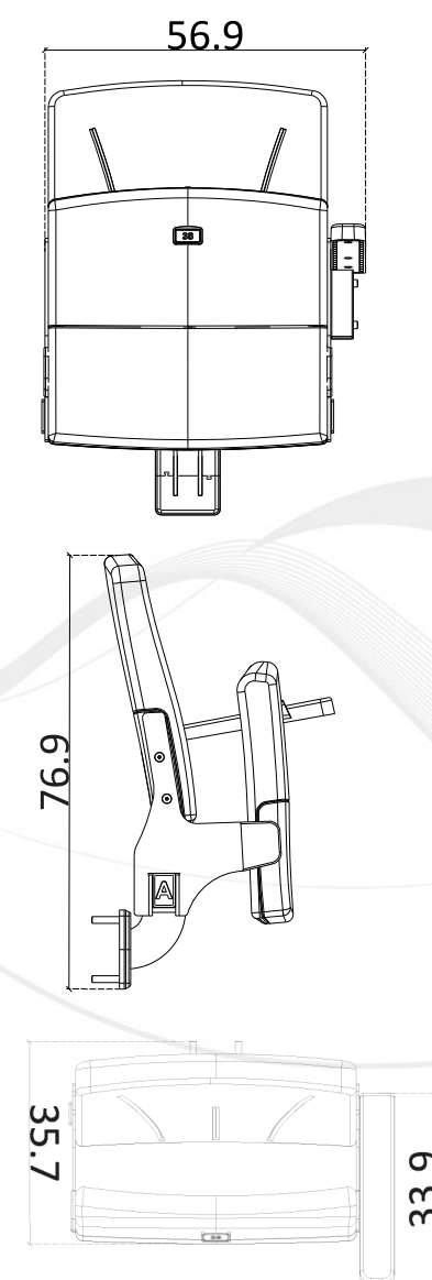
ROYAL-301 ON MONORAIL
