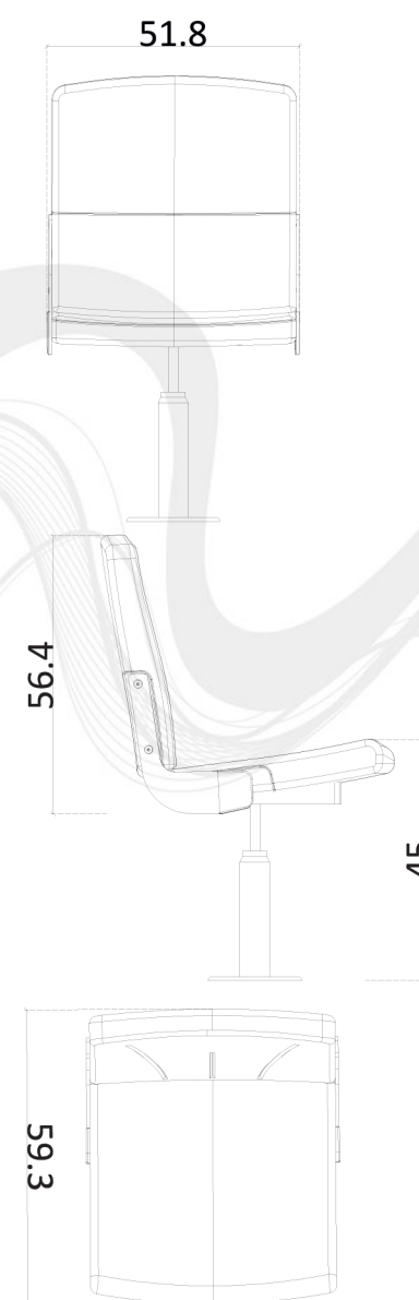
ROYAL-211 PRESS SEAT
