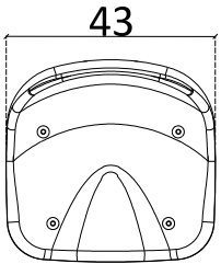
RISER MOUNTED-101
